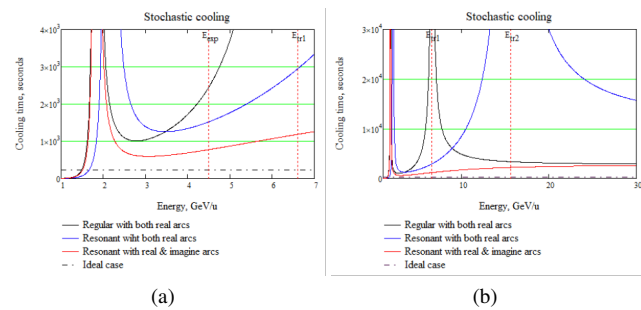
Fig. 5. (Color online) The dependence of stochastic cooling time on the energy for various lattices. Energy range (a) 1–7, (b) 0–30 GeV per nucleon.
